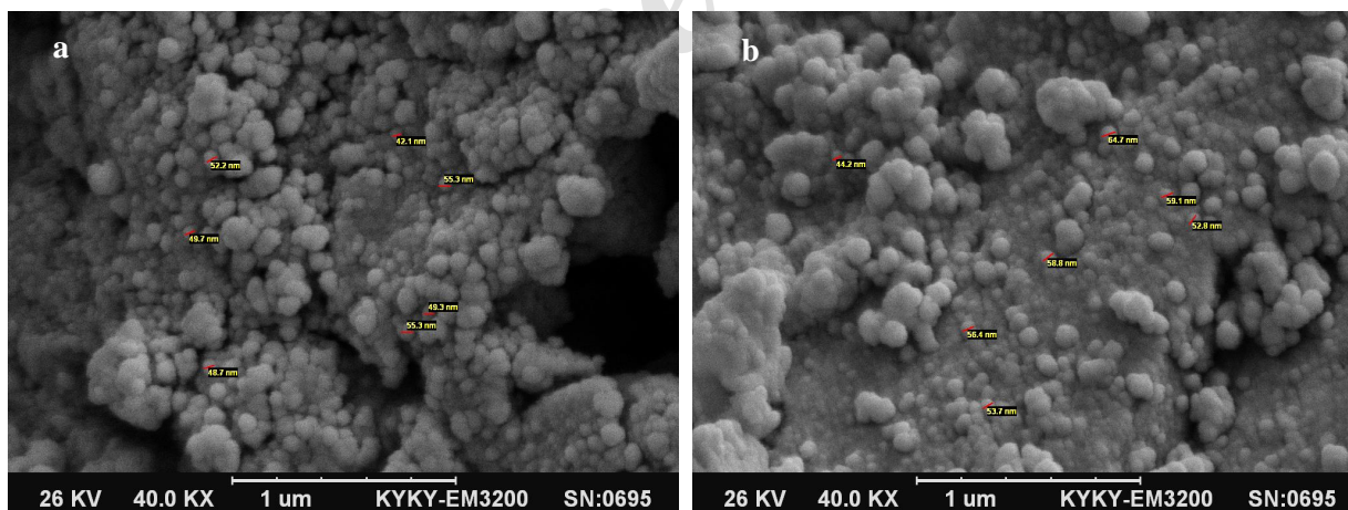
Figure 3: SEM images of prepared samples: (a) TiO 2 ; (b) 5-SA-TiO 2 .
