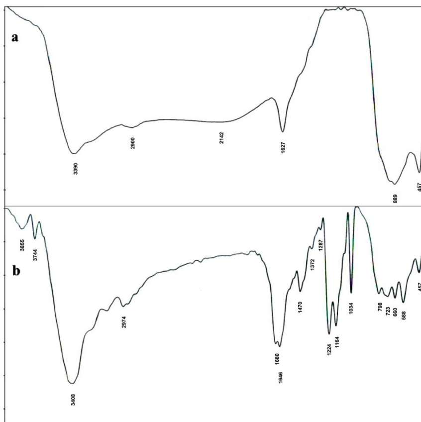
Figure 2: FT-IR spectra of prepared samples: (a) TiO 2 ; (b) 5-SA-TiO 2 .
