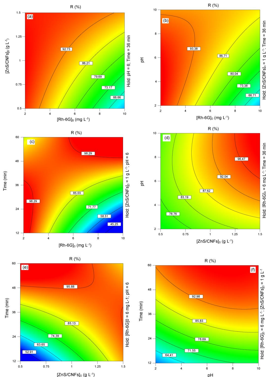
Figure 4: Counter plots of removal efficiency (%) as a function of (a) initial Rh-6G concentration and ZnS/CNFs concentration; (b) initial Rh-6G concentration and pH; (c) initial Rh-6G concentration and irradiation time; (d) ZnS/CNFs concentration and pH; (e) ZnS/CNFs concentration and irradiation time; (f) pH and irradiation time
