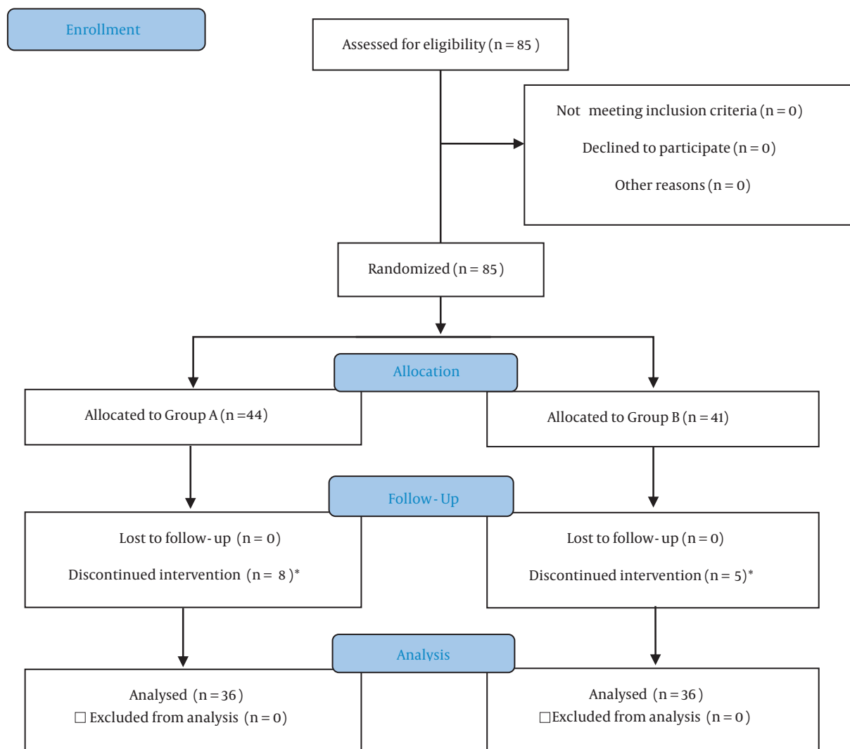
Figure 1. Consort diagram
