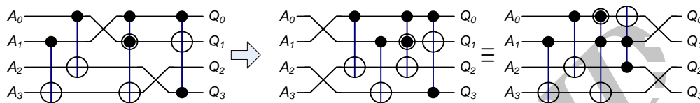
Figure 3. Using Swap gates to change the location of garbage outputs: (a) Swap gates are anywhere in the circuit, (b) Swap gates are moved to the input side, (c) Swap gates are moved to the output side.
