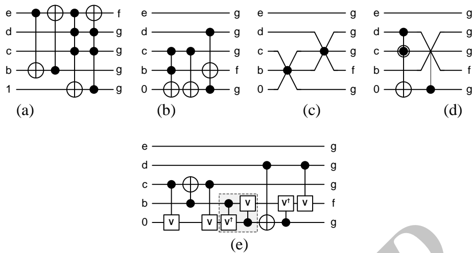
Figure 4. Proposed circuits for the 4gt5 benchmark: (a) circuit synthesized in [8], (b) optimized circuit using NCT gate library, (c) optimized circuit using generalized Fredkin gate library, (d) optimized circuit using a mixed gate library, (e) optimized circuit using a quantum VVP gate library.
