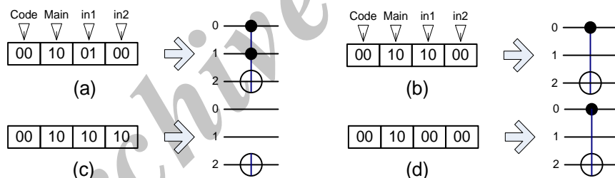
Figure 1. The method used for coding a reversible gate and different combinations of locations of inputs: (a) distinct locations, (b) the locations of a main input and a control input are the same, (c) all inputs have the same location, (d) all control inputs have the same location.
