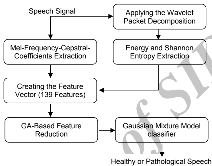
Figure 1. The scheme of the proposed method for detection of vocal fold pathology
