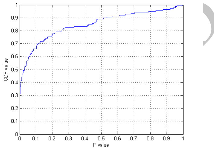
Figure 2. The P-value for features
