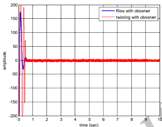
Figure 7. Control effort
