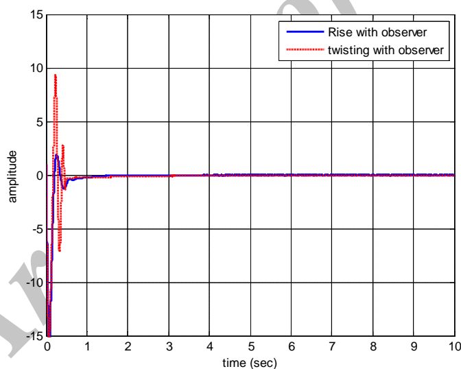
Figure 6. State x_2 applying Rise feedback controller in comparison with twisting algorithm
