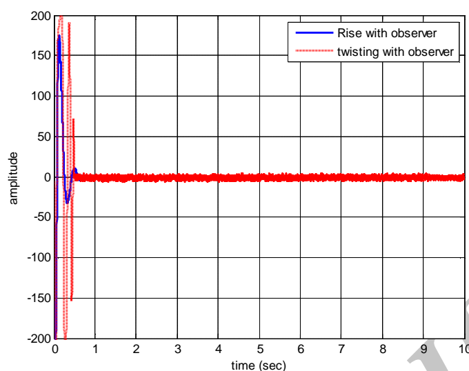
Figure 7. Control effort
