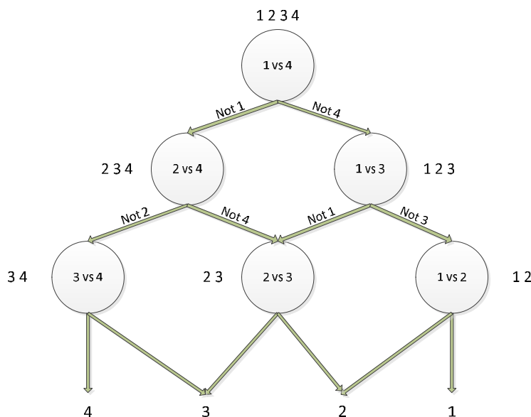
Figure 3. DAG method proposed in [14]
