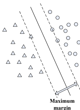
Figure 1. Finding the maximum margin by SVM
