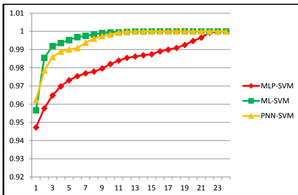
Figure 6. The probability of the presence of the correct character when choosing more than two probable characters
