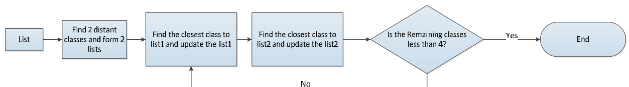
Figure 5. The flowchart of clustering algorithm
