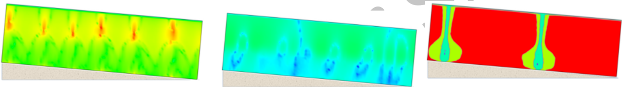
Fig. 2c: Contours of curvature at 6000 s from left to right for: Ri = 0.06, 0.2 and 0.3 . The maxima of this field correspond to critical points.
