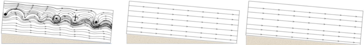
Fig. 2b: The stream function field at 6000 s from left to right for: Ri = 0.06, 0.2 and 0.3 . Sample elliptic and hyperbolic points are shown by circles and plus signs respectively.
