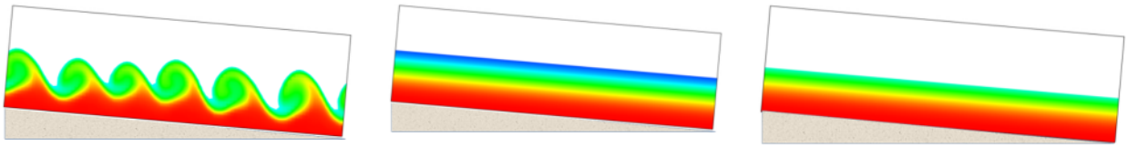
Fig. 2a: Contours of density difference \rho - \rho_0 at 6000 s from left to right for: Ri = 0.06, 0.2 and 0.3 . Small values are brought colorless.
