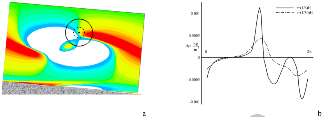
Fig.4, a: Contours of the temporal differenced density at 4000 s. Values less than 0.002\text{kg}/\text{m}^3 are brought colorless for more clarity, b: Values of the temporal differenced density on circles of the left panel with respect to the sampling angle.
