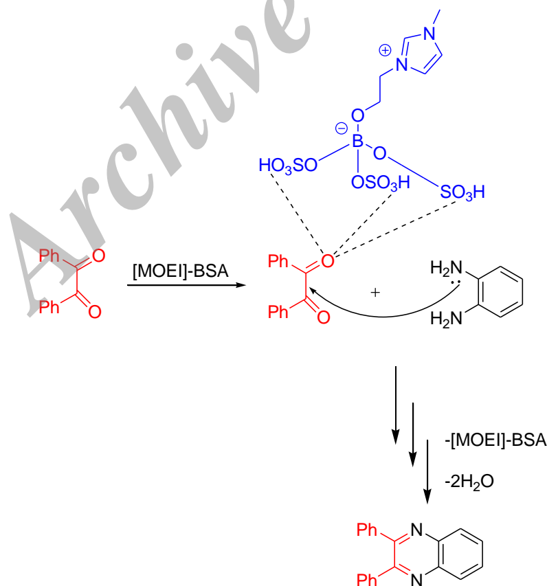
Scheme 3. Proposed mechanism of catalyst.
