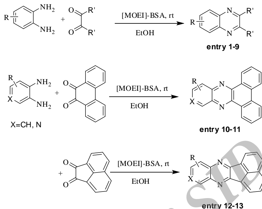
Scheme 1. Quinoxaline synthesis using [MOEI]-BSA.
