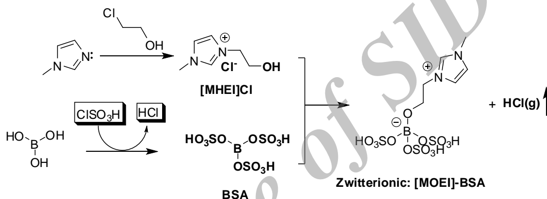
Scheme 2. Synthesis of [MOEI]-BSA as a catalyst.
