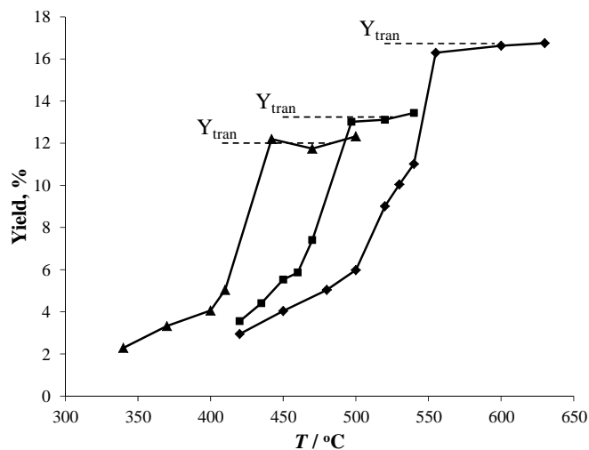
Fig. 6. Propene yield variation with temperature. Reaction condition: GHSV = 60000 \text{ cm}^3 \text{ gr}^{-1} \text{ hr}^{-1} , Feed composition: N_2/O_2/C_3 = 8/1/1 (◆: VAI-01, ■: VAI-02, ▲: VAI-03).
