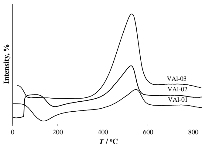
Fig. 3. TPR pattern of the catalyst samples.
