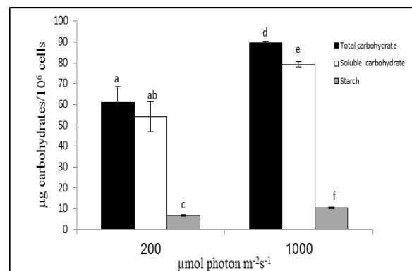
Fig. IV. Effect of light intensity on carbohydrates content of D. salina
