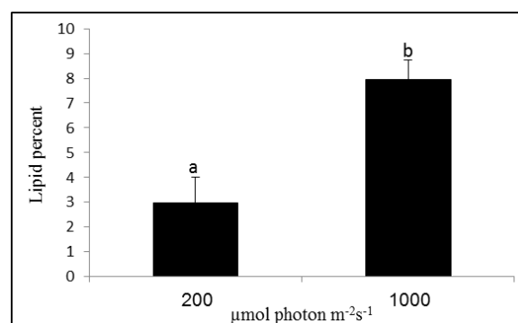
Fig. VI. Effect of light intensity on lipids percent form total dry weight of D. salina
