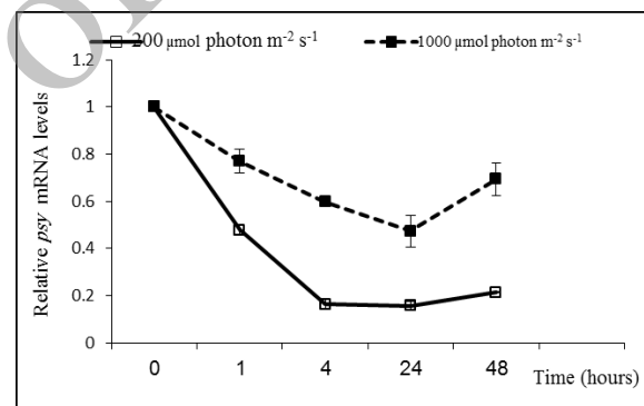
Fig. III. Effect of light intensity on relative psy mRNA levels of D. salina
