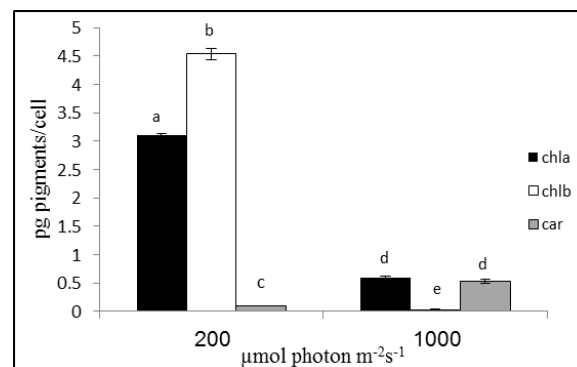
Fig. II. Effect of light intensity on D. salina pigments content
