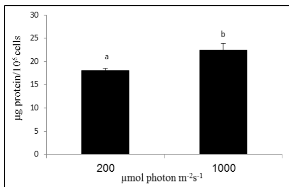
Fig. V. Effect of light intensity on total proteins content of D. salina
