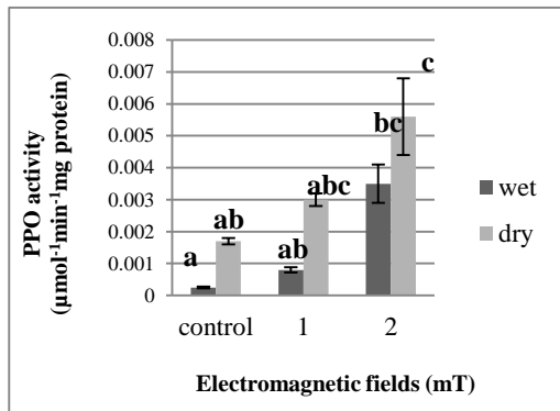
Fig. VIII. Effect of the electromagnetic fields on PPO activity in Valerian ( V. officinalis L.). PPO activity exposure to electromagnetic fields. Data are presented as the means \pm SE. Means followed by different letters represent significant difference at P < 0.05 according to post hoc Tukey's test.
