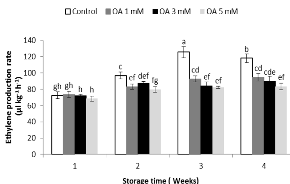
Fig. I. Effect of oxalic acid treatment (0, 1, 3, and 5 mM OA) on ethylene production of peach fruit stored at 1^\circ \text{C} for 4 weeks; data shown are mean values \pm SE ( n = 3 ). Data followed by different letters are significantly different according to Duncan's multiple range test, P < 0.05 .
