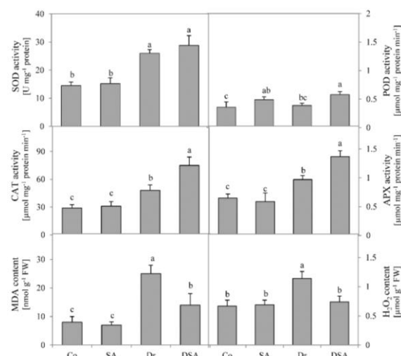
Fig. III. Antioxidant index of S. nemorosa plants under different treatments; SOD: superoxide dismutase; CAT: catalase; POD: peroxidase; APX: ascorbate peroxidase; MDA: malondialdehyde; H_2O_2 hydrogen peroxide; each value is the mean \pm SD of 4 replicates. Bars indicated with the same letter are not significantly different ( P < 0.05 ).
