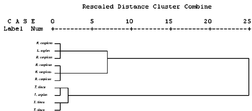
Figure 5. Dendrogram derived from cluster analysis of the elemental concentrations of the fish liver and kidney between habitats in the coastal water of the Iranian Caspian Sea, Cluster analysis, as a complementary method, divided the fish into two sub-groups. No variation was found for element concentrations in Roach and Asp, while Tench was placed in a distinct subgroup, this graph obtained by SPSS version 16.0.
