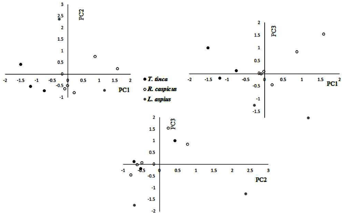
Figure 2. Principal component analysis (PCA) of elemental concentrations of the fish liver and kidney between habitats in the coastal water of the Iranian Caspian Sea. Scatter plots demonstrate individual fish scores for PC1 vs. PC2, PC1 vs. PC3, and PC2 vs. PC3 which together explain 83.60% of the total variance, this graph obtained by SPSS version 16.0.
