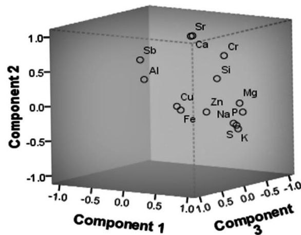
Figure 3. Characteristic load for PC1, PC2 and PC3 obtained by multi-elemental principal components analysis (PCA) for the elemental concentrations of the fish liver and kidney between habitats in the south Caspian Sea water, this graph obtained by SPSS version 16.0.
