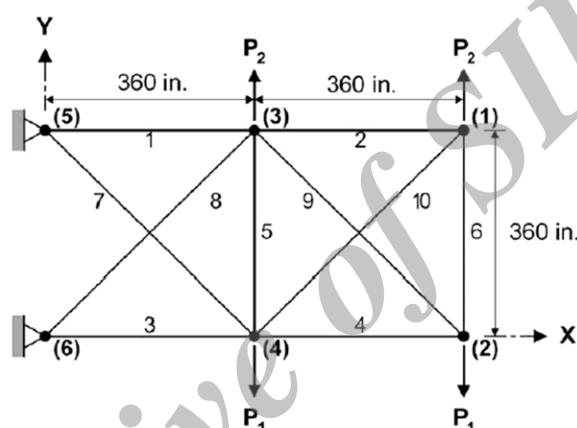
Figure 4. 10-bar planar truss
