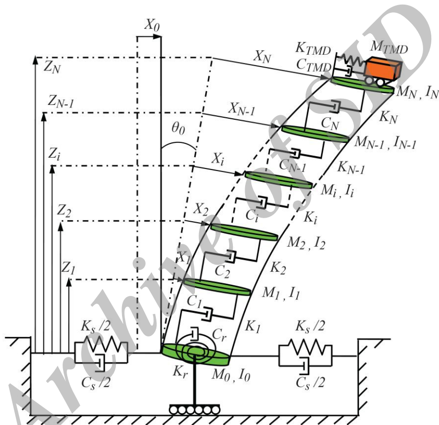
Figure 1. Shear building configuration
