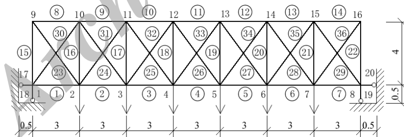
Figure 1. A 40-bar planar truss
