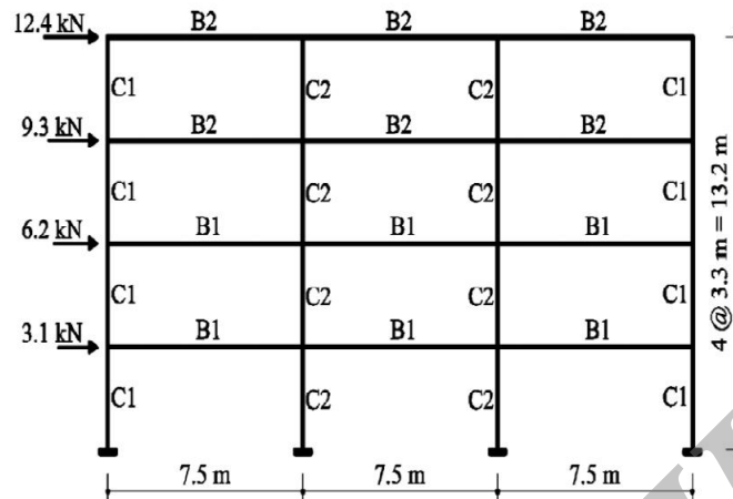
Figure 5. Three bay, four-story RC frame
