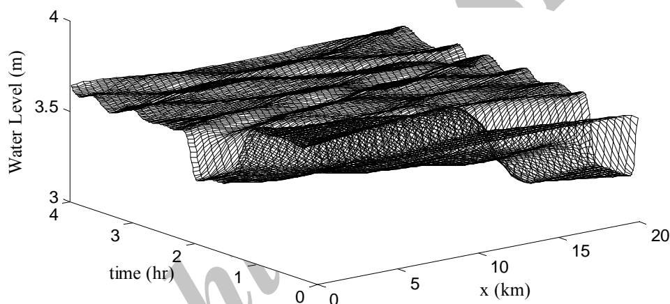
Figure 9. A 3D view of water level fluctuations in the whole channel over simulation time when the control found in this study (solid line in Figure 7) is imposed at upstream end ( f=1015.58\text{ m} )
