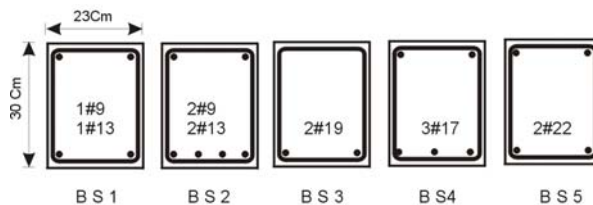
Figure 2. Detail of beams with longitudinal steel
