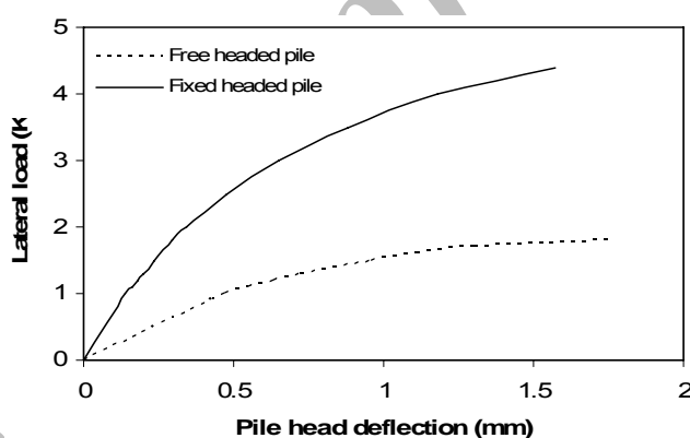
Figure 5. Computational load-deflection curves [5]
