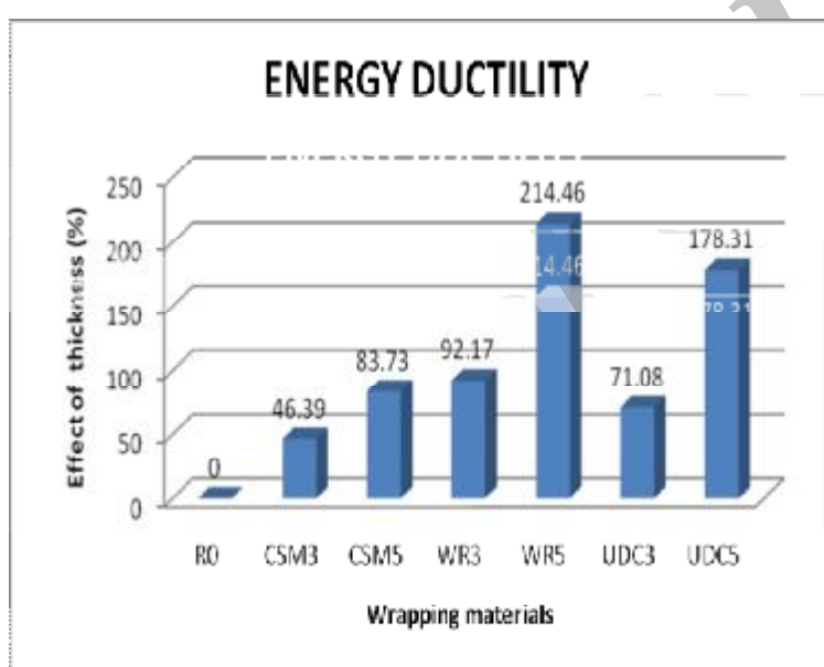
Figure 10. Energy ductility for the specimens
