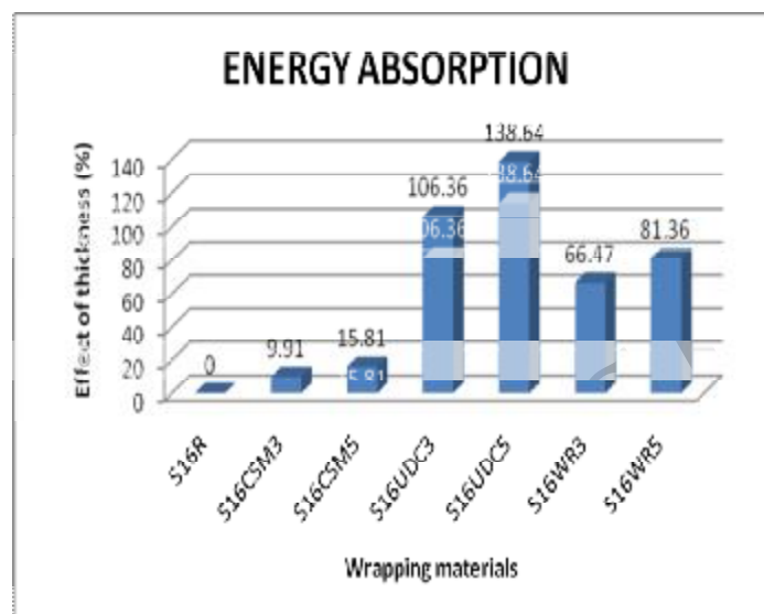
Figure 11. Energy absorption for the specimens
