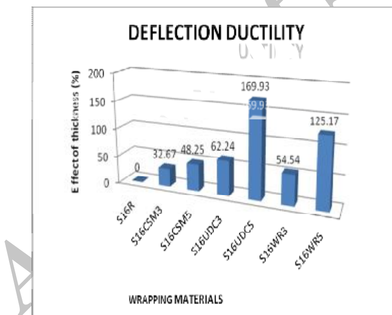
Figure 9. Deflection ductility for the specimens
