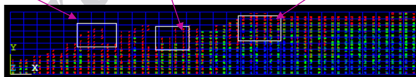
Figure 15. Integration of all cracks at 49.00kN for FRP Beam 1
