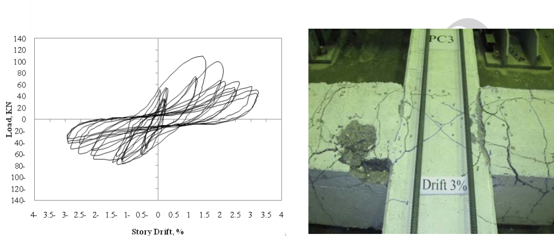
Figure 10. Lateral load versus story drift response for specimen PC3 (Left) Damage in specimen PC3 at 3% drift angle (Right)
