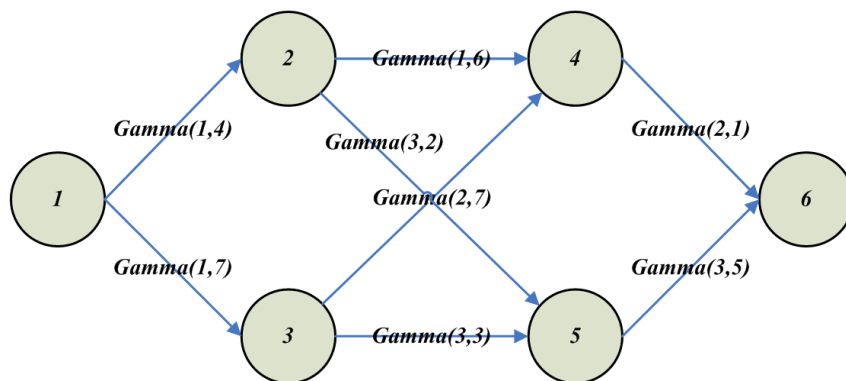
Fig. 2 A network with gamma distribution arc length
