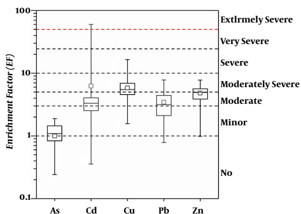
Figure 3. Boxplot of enrichment factor for heavy metals in street dust from Tehran. No enrichment ( EF \leq 1 ); minor enrichment ( 1 < EF \leq 3 ); moderate enrichment ( 3 < EF \leq 5 ), moderately severe enrichment ( 5 < EF \leq 10 ), severe enrichment ( 10 < EF \leq 25 ), very severe enrichment ( 25 < EF \leq 50 ), and extremely severe enrichment ( EF > 50 ).
