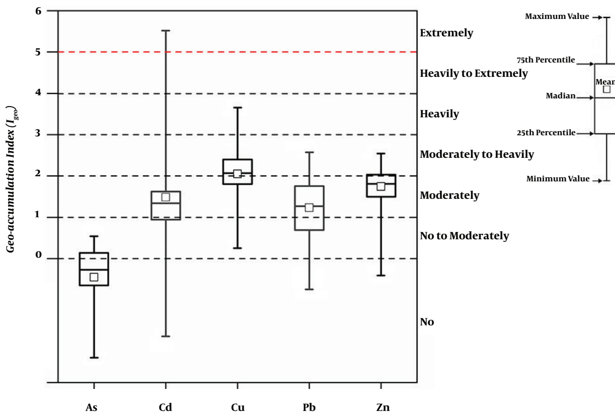
Figure 2. Boxplot of geo-accumulation index for heavy metals in street dust from Tehran. No pollution ( I_{geo} \leq 0 ); no to moderate polluted ( 0 < I_{geo} \leq 1 ); moderately pollution ( 1 < I_{geo} \leq 2 ), moderately to heavily polluted ( 2 < I_{geo} \leq 3 ), heavily polluted ( 3 < I_{geo} \leq 4 ), heavily to extremely polluted ( 4 < I_{geo} \leq 5 ), and extremely polluted ( I_{geo} > 5 )
