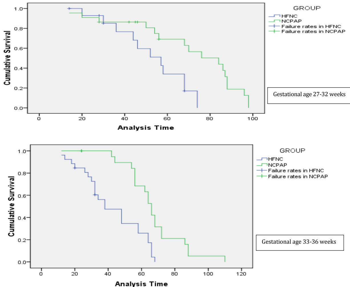
Figure 2. Kaplan-Meier Estimate
