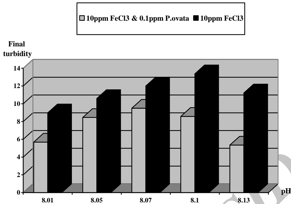
Fig 2. Comparison of final turbidity in two following conditions: using chloroferic coagulant alone and using chloroferic coagulant together with P. ovata coagulant aid in turbidity of 50 and pH 8.
