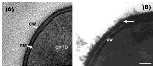
Figure 4. The cell wall structure of (A): S. pneumoniae 20 with permission and (B): S. aureus 21 with permission. CW: cell wall, PM: plasma membrane, Bar = 100μm.
