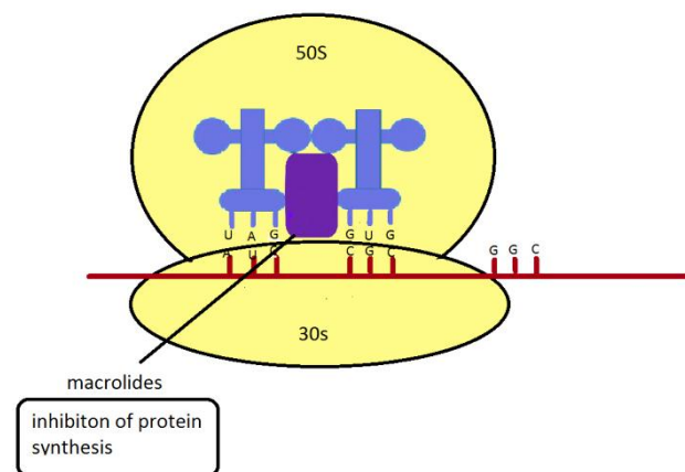
Figure 1. Schematic representation for antibacterial mechanism of macrolides.
