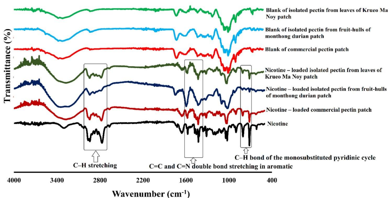
Figure 4. FTIR spectra of nicotine transdermal patches made from commercial pectin and isolated pectin
