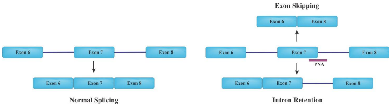
Figure 5. Splicing pattern of pre mRNA. Left: Normal splicing is shown by joining of exons to generate a spliced mRNA transcript. Right: Modification of splicing by antisense PNAs leading to exon skipping or intron retention. Blue rectangles, exons; lines, introns.
