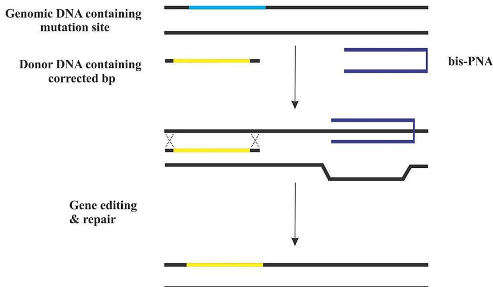
Figure 6. Schematic illustration of PNA-mediated gene editing. Triplex forming PNA can distort helical structure of DNA, inducing endogenous DNA repair in presence of DNA donor containing corrected nucleobases. The ability of PNAs in gene editing and repair comes directly from binding to cognate sites, provoking endogenous editing system. 81
