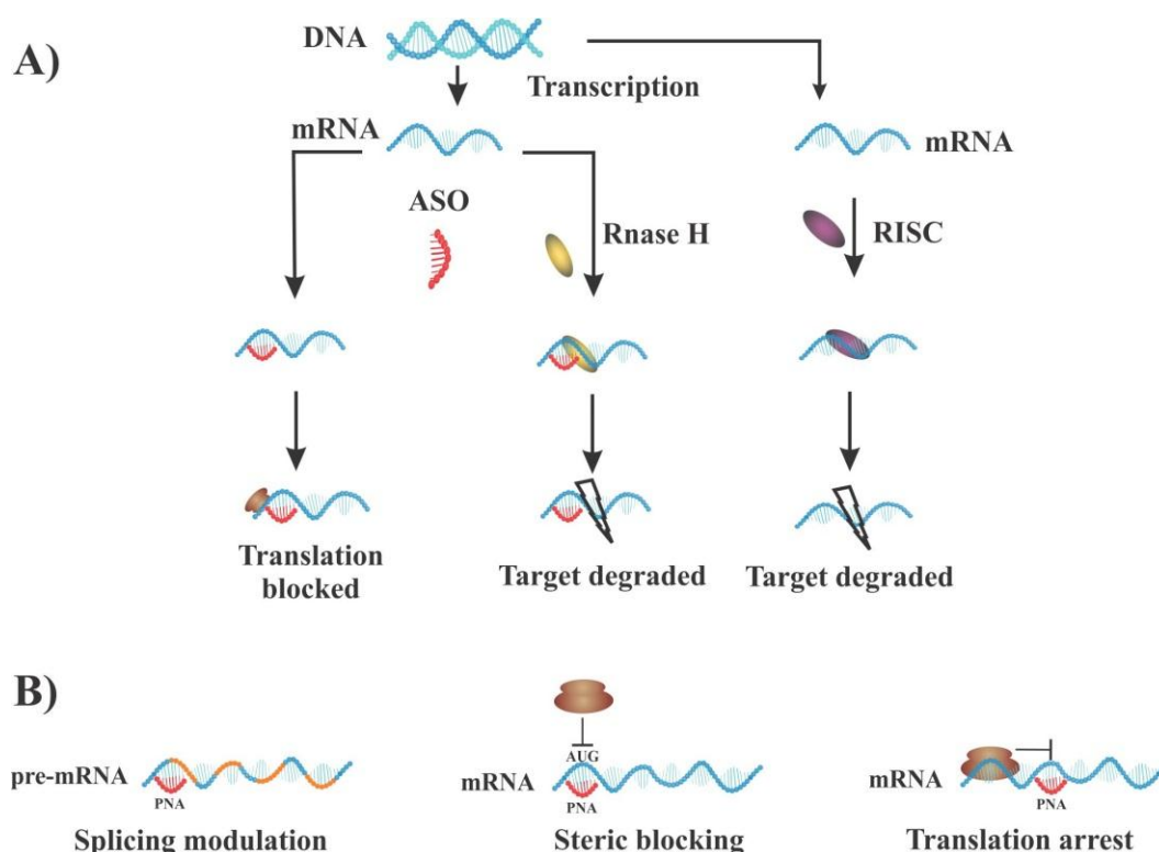
Figure 4. Some mechanisms involved in modulation of gene suppression: A) Antisense activity and RNA interference mechanisms. B) Inhibitory effect of antisense PNA via different approaches. PNAs have the ability to target AUG regions (translational start codon) or 5'UTR, where the starting point of ribosomal assembly occurs and block process, whereas triplex forming PNAs can inhibit elongation process via targeting to coding region. ASO: antisense oligonucleotide.
