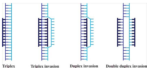
Figure 2. Schematic drawing of PNA binding modes, targeting to dsDNA. DNA is drawn as a ladder and PNA molecules are in thick structures. Triplex complex is formed by cytosine rich PNA targeting to homopurine target. Triplex invasion structure leads to the formation of a loop. In this structure, one strand of PNA binds based on Watson-Crick rule, and another strand binds through Hoogsteen bond. Duplex invasion has no sequence constraints. Double duplex invasion is formed by PNAs containing modified bases. 3
