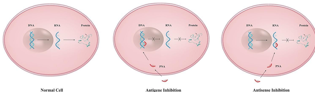
Figure 3. Schematic illustration of PNA-based strategy as antigene and antisense agents. Antigene PNA binds to complementary sequence in DNA and inhibits transcriptional process while antisense PNA hybridize to target sequence in mRNA and prevent translation procedure.
