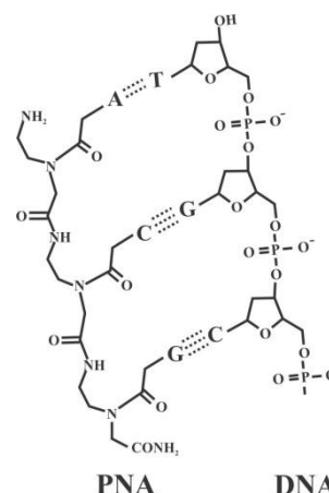
Figure1. Comparison of chemical structure of PNA and DNA backbones. 2
