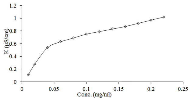
Figure 1. Change of conductivity with increasing SOD-CAS concentration.
