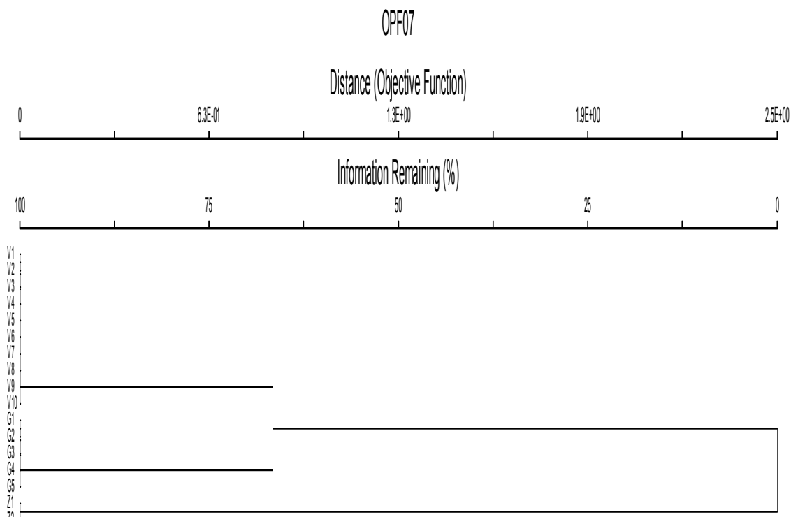
Fig. 6: Dendrogram created by UPGMA algorithm using Jaccard similarity coefficient on data from primer OPF-07 for 17 populations of Chara (V1-V10: 10 populations of C. vulgaris , G1-G5: five populations of C. gymnophylla and Z1-Z2: two populations of C. zeylanica ).
