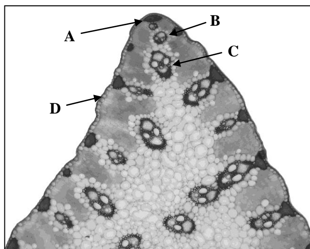
Fig. 3. Stem anatomical parts in Bolboschoenus genus: A, Sclerenchyma strand; B, Small vascular bundle; C, Large vascular bundle; D, Epiderm (translucent cells)
