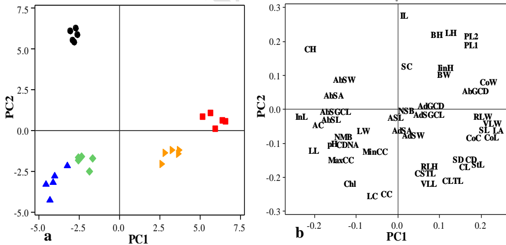
Fig. 2. Scatterplot of first two components from a PCA performed with 46 variables of 25 specimens. Different symbols indicate grouping by different functional classifications: a, five Satureja species, S. bachtiarica (●); S. khuzistanica (■); S. spicigera (◆); S. sahendica (▲) and S. rechingeri (►). b, Morphological traits (refer to table 2 for full names of all traits).
