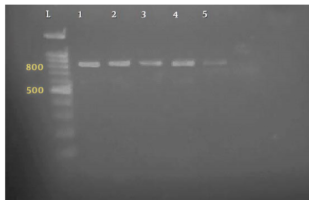
Figure 1. Electrophoresis of PCR product of Cryptosporidium parasites, based on SSUrRNA gene on 1% agarose gel. DNA marker (leader) 100 bp. Line 1 standard sample, line 2-5 samples of the patients (824 - 864 bp).
