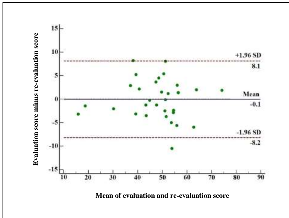
Fig. 2. Bland-Altman plot showing the average against the difference between evaluation and re-evaluation scores of the Persian tinnitus functional index total score.
