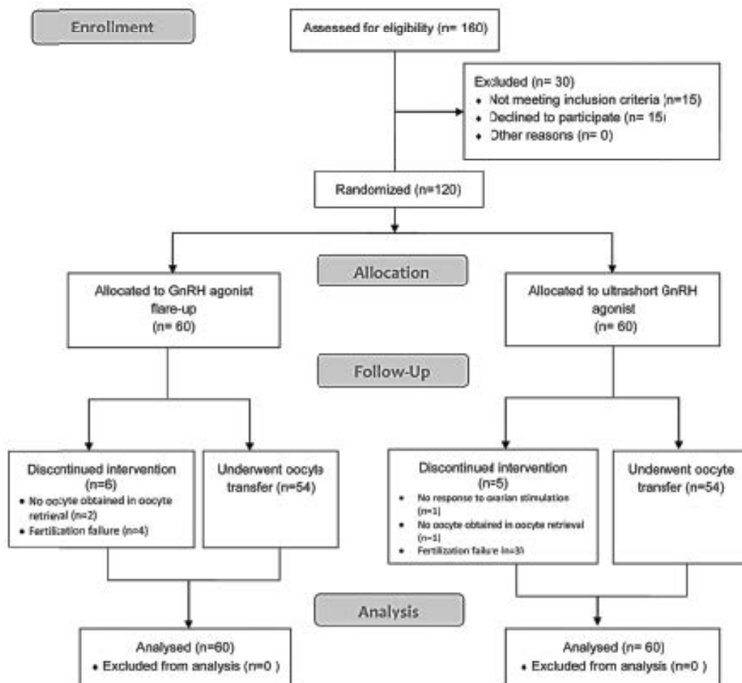
Fig 1: Study flowchart.
