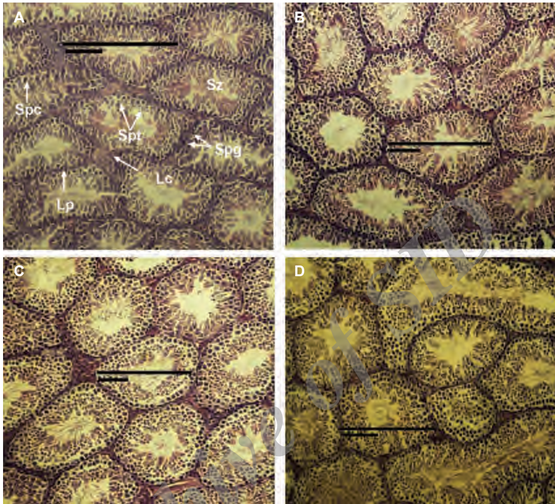
Fig.2: Microscopic images of testis slides of embryo groups (H & E, \times 400 ). A-D. Control and treatment groups receiving 10, 20, and 40 mg/kg CdSe: ZnS. Sz; Spermatozoa, Lc; Leydig cells, Lp; Lamina propria, Spg; Spermatogoni, Spc; Spermatocytes and Spt; Spermatids.
