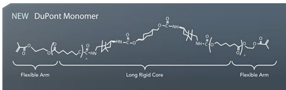
Figure 1: DX-511 monomer
