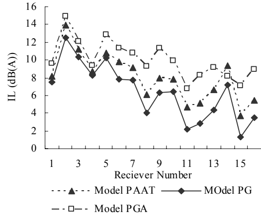
Fig. 15. The A-weighted mean insertion loss for diffusive parallel barrier model PGA along with its equivalent partially diffusive barrier model PG and fully absorbent barrier model PAAT at 16 receiver points
