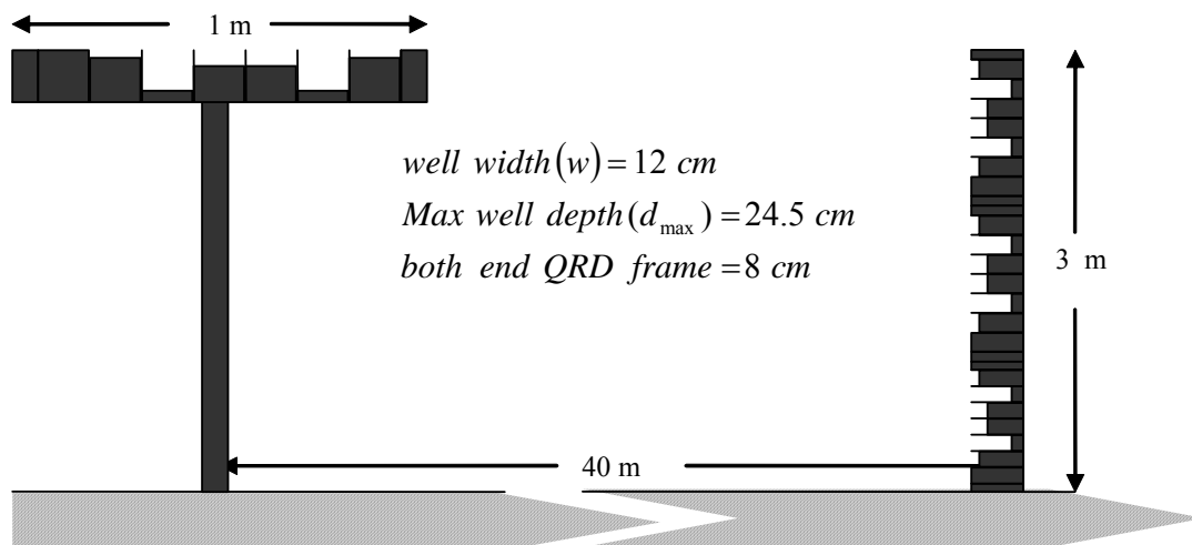
Fig.3 . Dimensions of the T-shape barrier (barrier No.1) having a QRD ( N = 7^* and fr = 400 \text{ Hz} ) and the vertical barrier No.2 having 3 QRDs ( N = 7 and fr = 400 \text{ Hz} ) in parallel barrier model “PGG”
