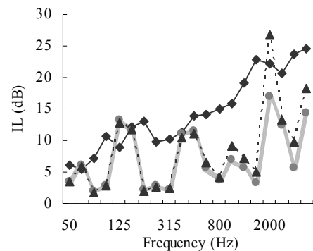
Fig. 6. Predicted frequency spectra of barrier insertion loss for two different parallel barriers along with their equivalent T shaped single barrier at the receiver point (-50,0)
