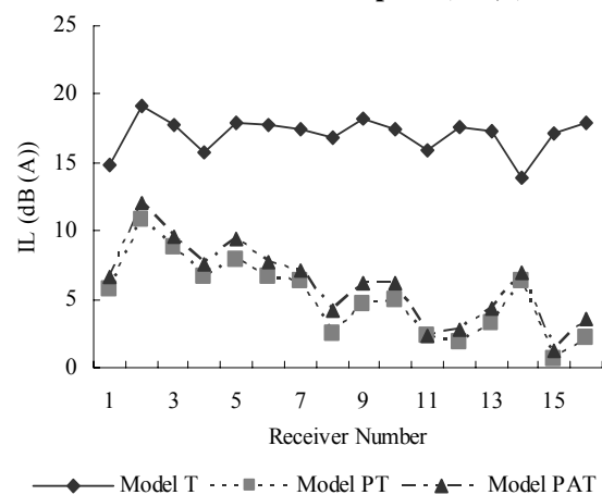
Fig. 7. The A-weighted mean insertion loss for two different parallel barriers along with their equivalent T shaped single barrier at 16 receiver points
