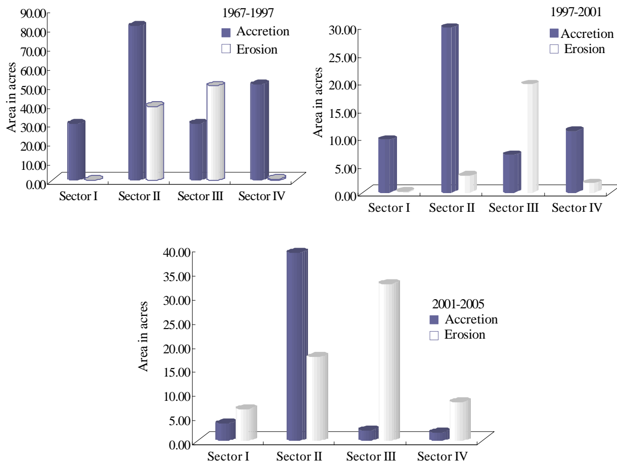
Fig. 3. Bar diagram showing rate of changes in areal extent of beaches during the last 38 years
