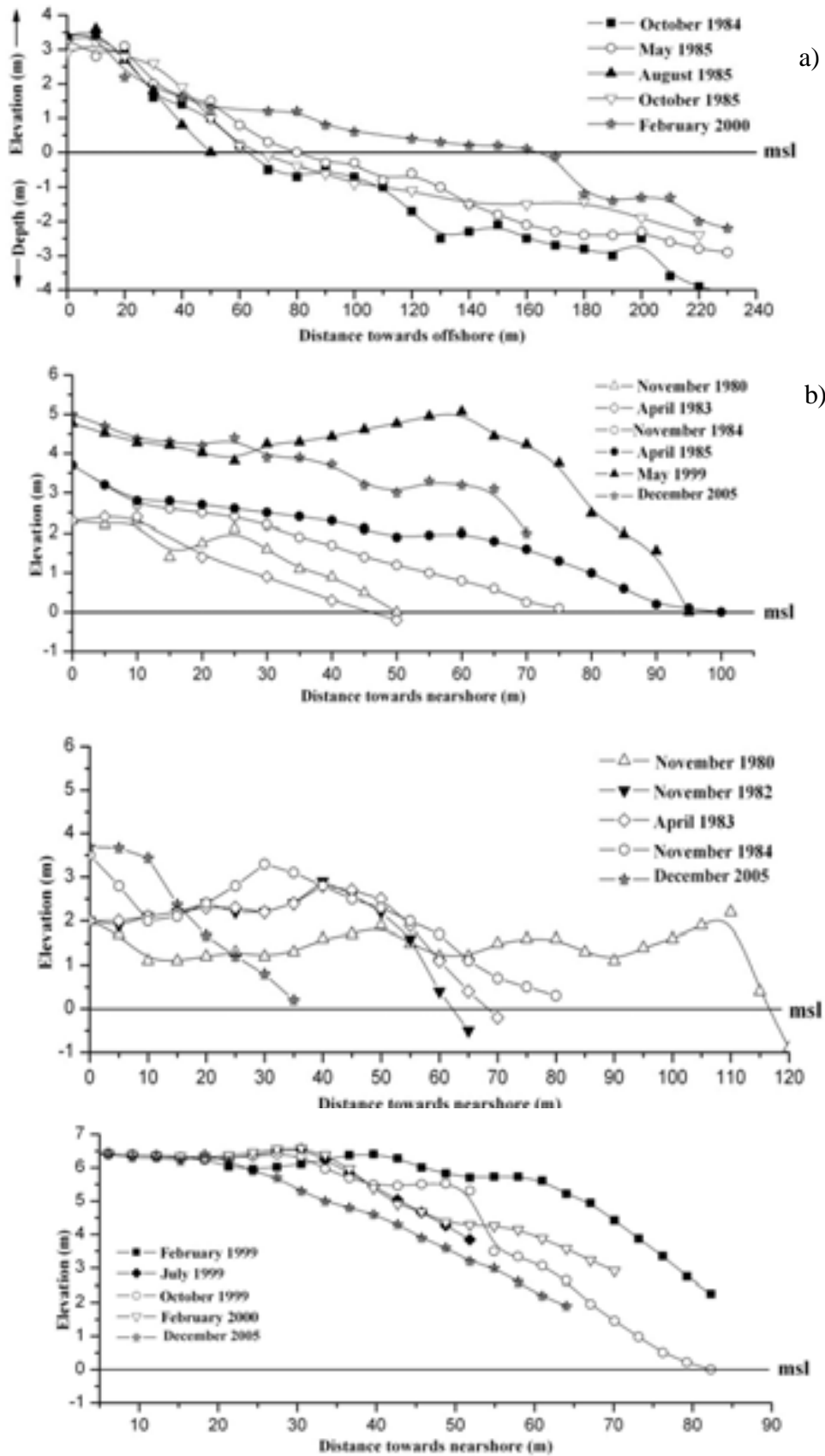
Fig. 4. Beach and nearshore profiles of Thannirbhavi (a). Beach profiles of Bengre (b); Kotepura (c); and Ulal (d)
