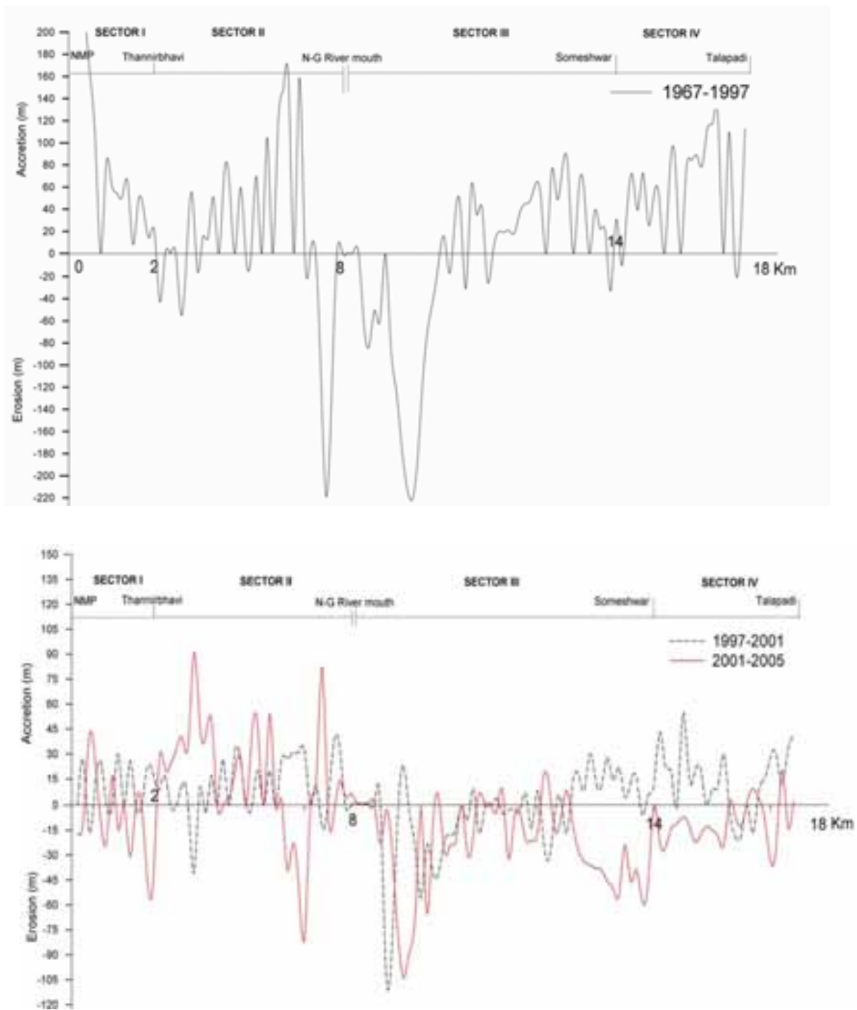
Fig. 2. Long-term (1967-1997) and short-term (1997-2001 & 2001-2005) changes in accretion and erosion patterns in all the four sectors
