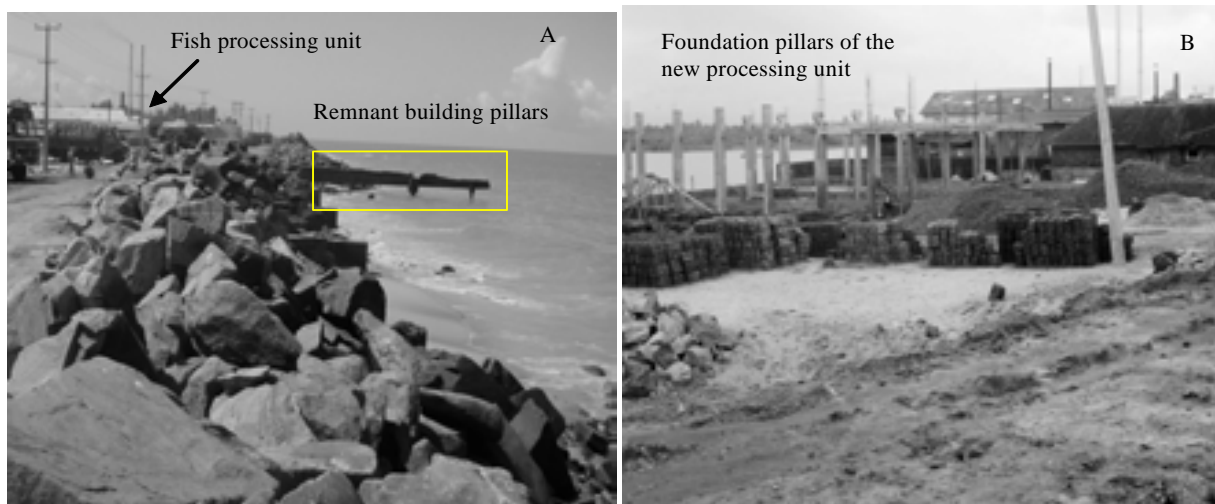
Plate 3. Establishment of fish processing unit and new building construction at the Ullal spit
