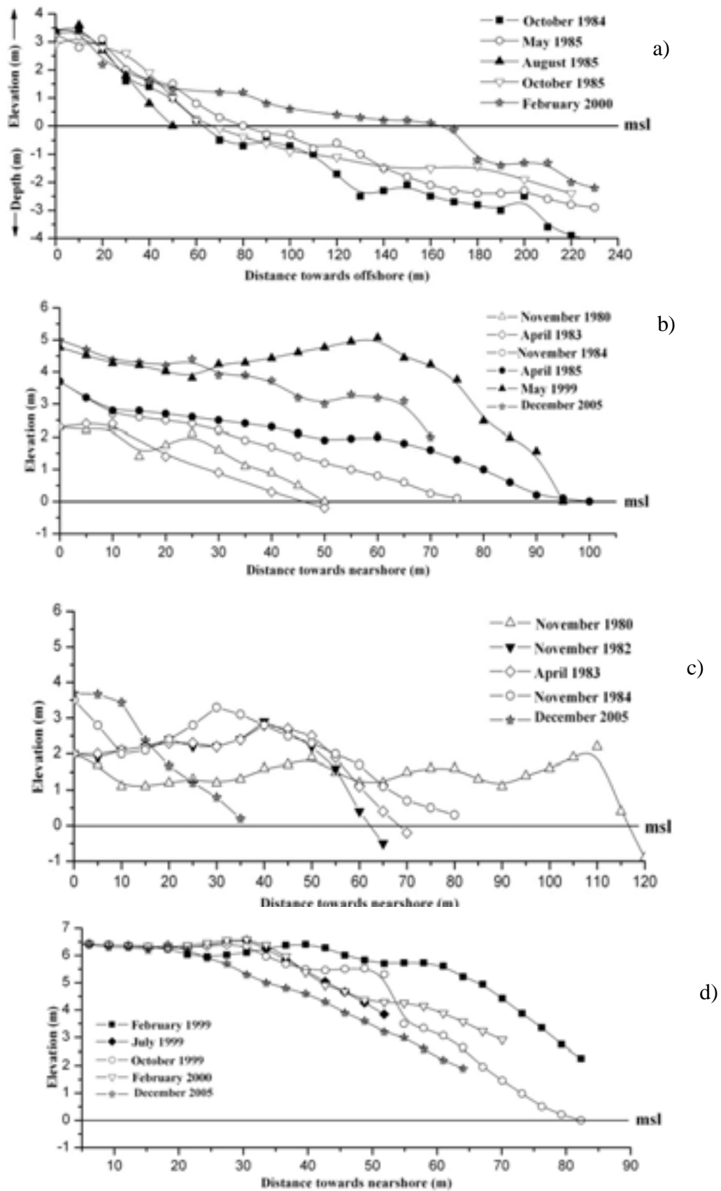
Fig. 4. Beach and nearshore profiles of Thannirbhavi (a). Beach profiles of Bengre (b); Kotepura (c); and Ullal (d)
