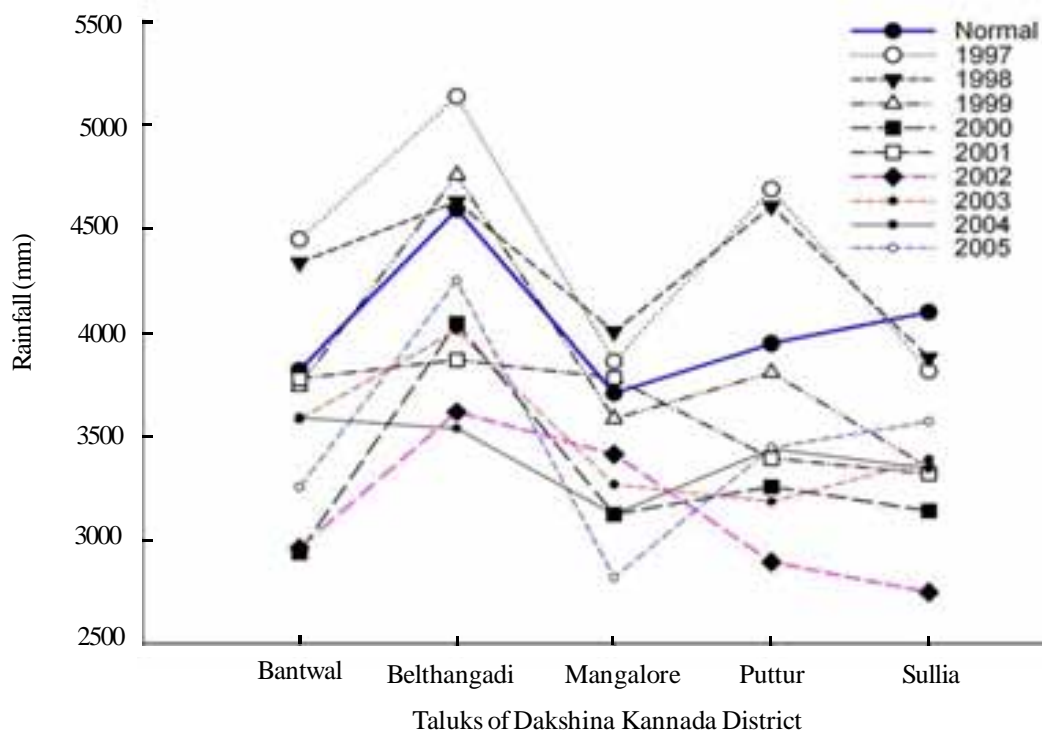
Fig. 5. Showing variation in the annual average rainfall for last 10 years (Source. Dakshina Kannada at a glance, 2006–2007)
