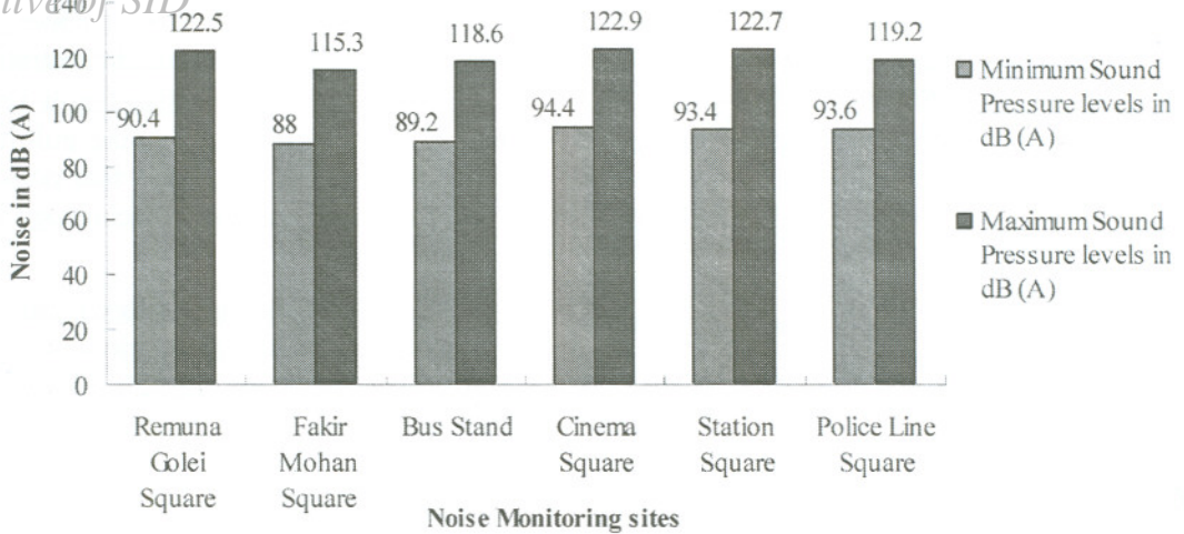
Fig. 3. Range of Noise levels in different noise monitoring sites at around Balasore, Orissa, India
