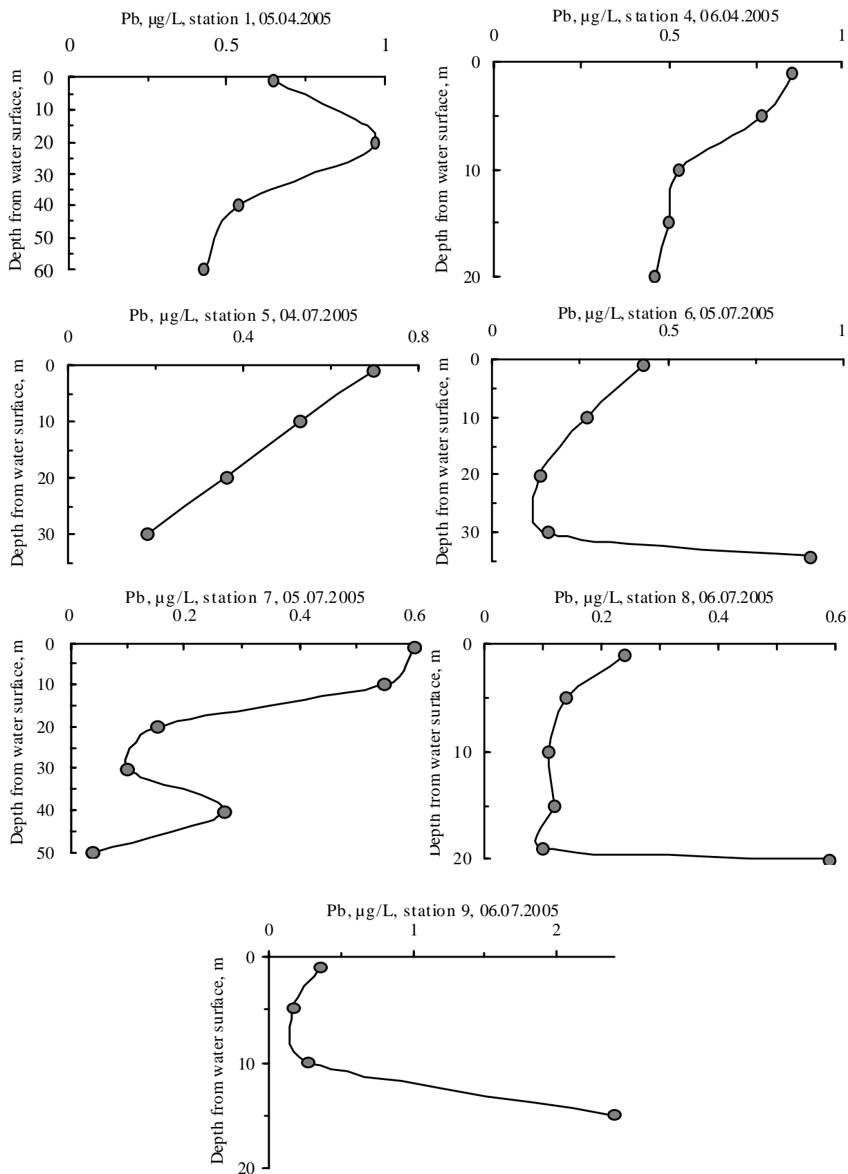
Fig. 2. Distribution of total concentration of Pb in water column of the sampling stations of Lake Umbozero (in µg/L)
