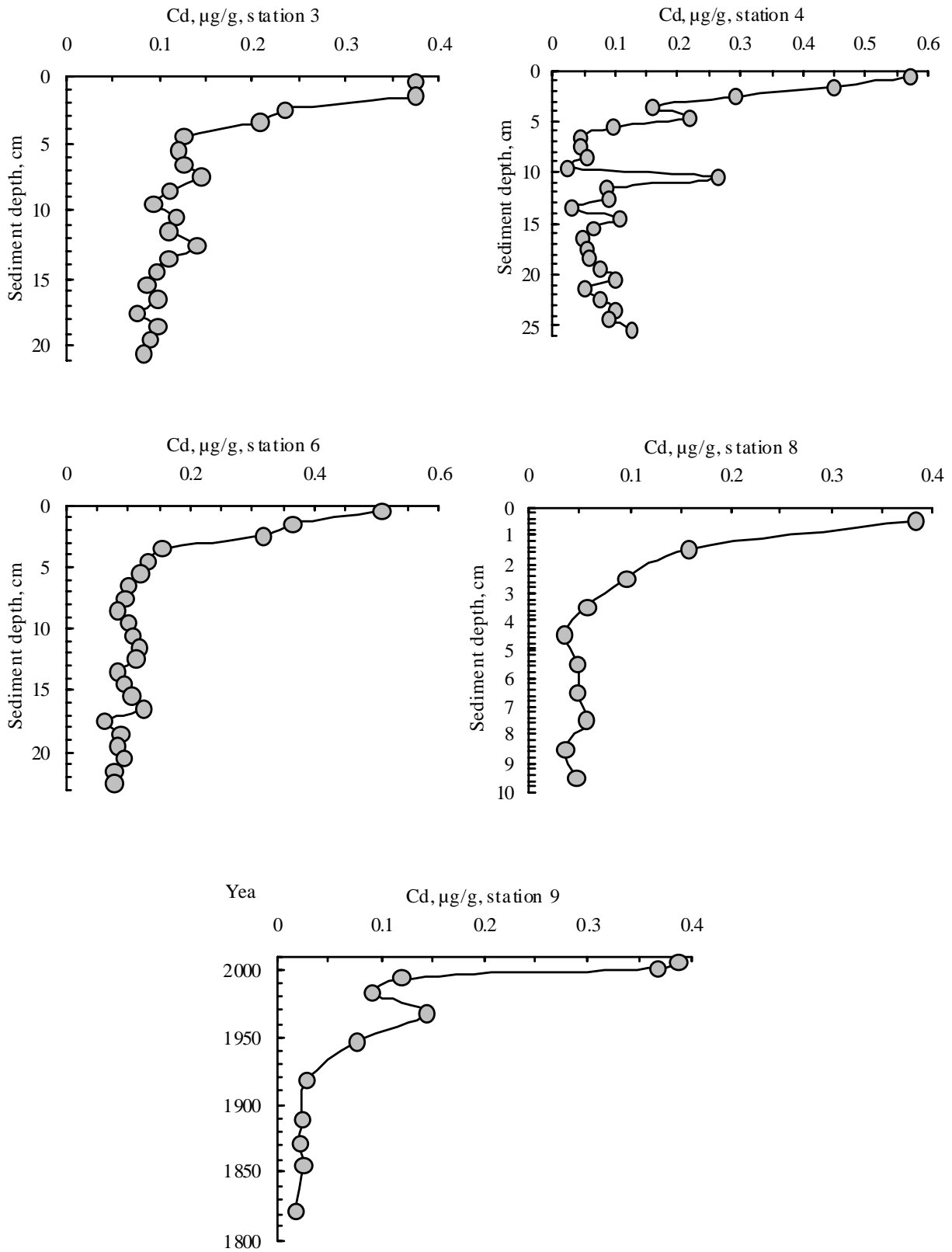
Fig. 5. Vertical distribution of Cd ( \mu\text{g/g} dry weight) in the sediment cores of the sampling stations of Lake Umbozero (for station 9 in dating sediment core)
