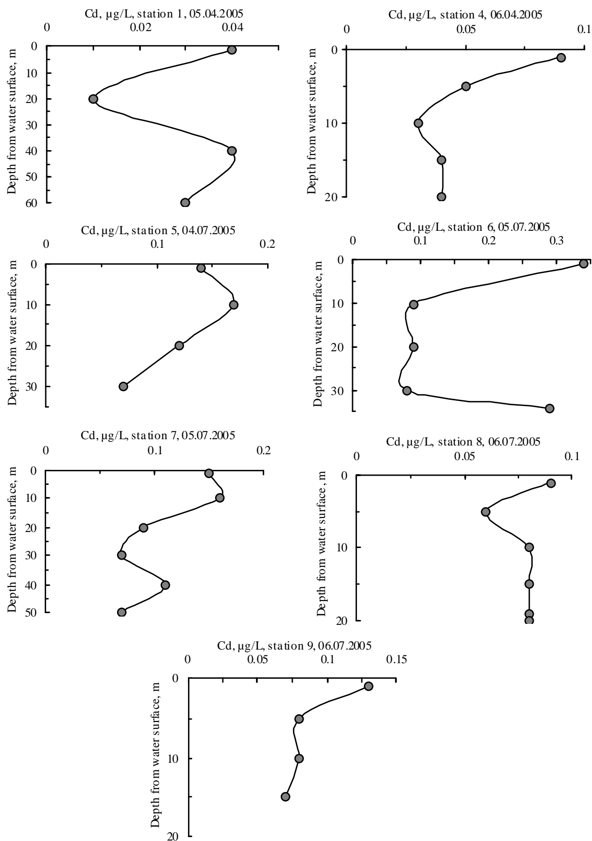
Fig. 4. Distribution of total concentration of Cd in water column of the sampling stations of Lake Umbozero (in \mu\text{g/L} )
