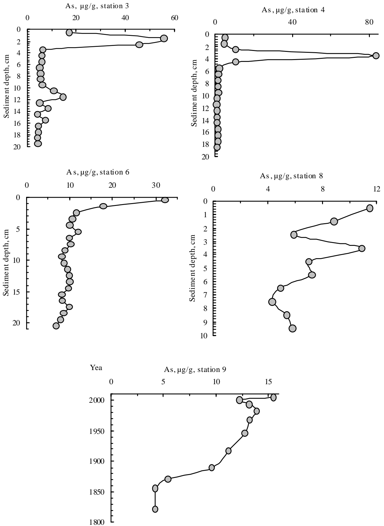
Fig. 7. Vertical distribution of As ( \mu\text{g/g} dry weight) in the sediment cores of the sampling stations of Lake Umbozero (for station 9 in dating sediment core)
