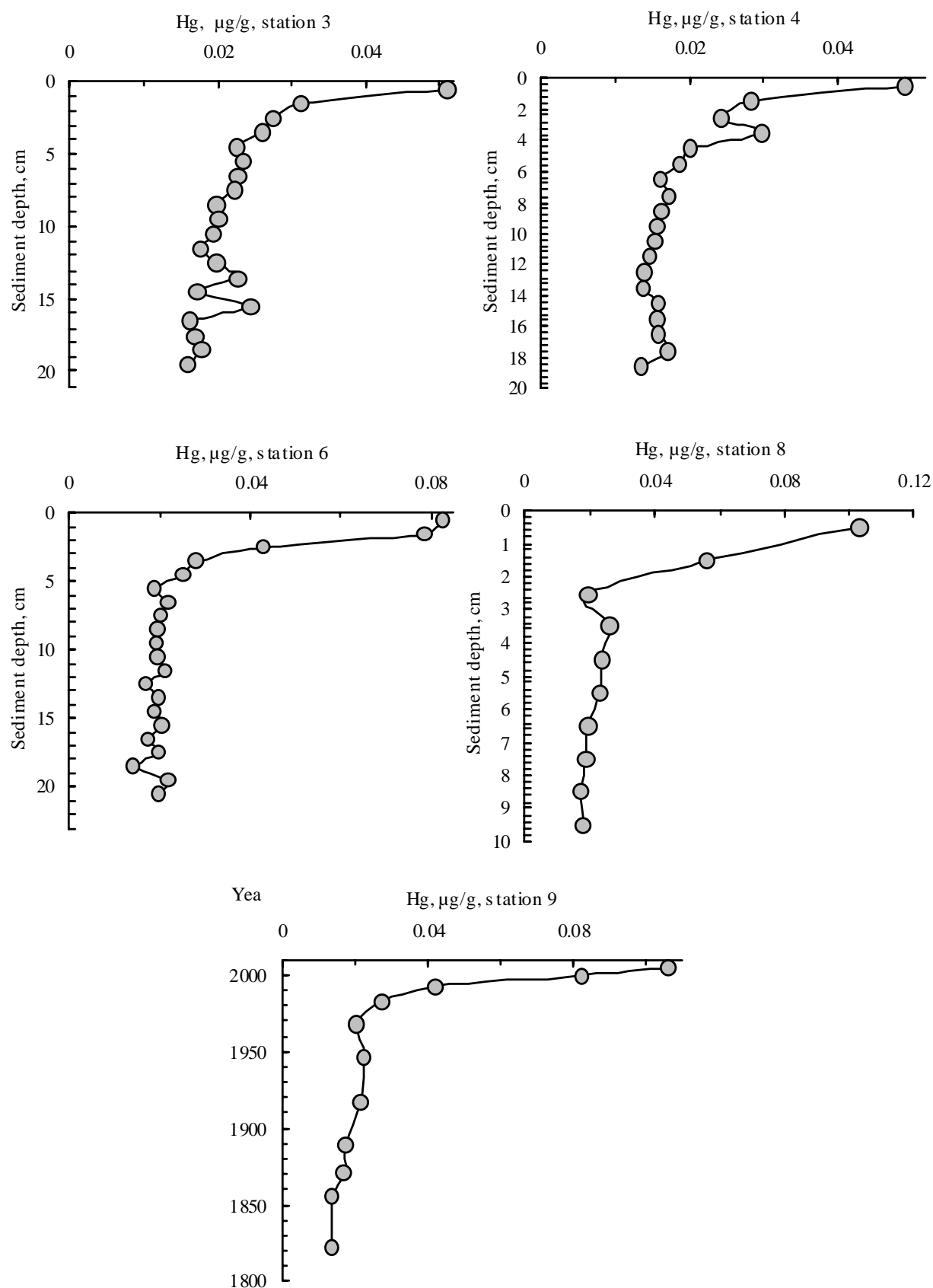
Fig. 8. Vertical distribution of Hg (μg/g dry weight) in the sediment cores of the sampling stations of Lake Umbozero (for station 9 in dating sediment core)
