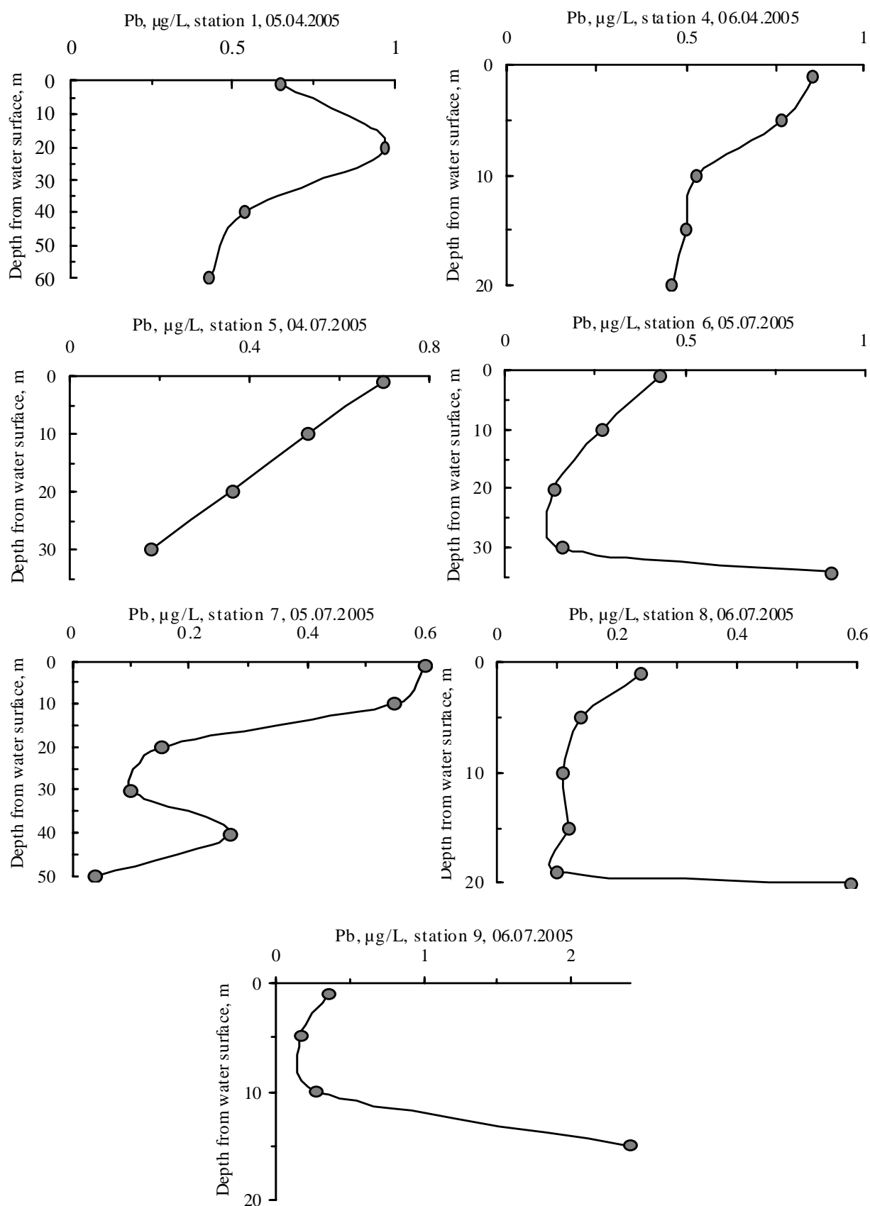
Fig. 2. Distribution of total concentration of Pb in water column of the sampling stations of Lake Umbozero (in \mu\text{g/L} )
