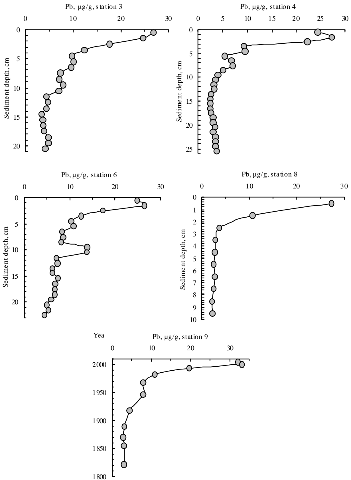
Fig. 6. Vertical distribution of Pb ( \mu\text{g/g} dry weight) in the sediment cores of the sampling stations of Lake Umbozero (for station 9 in dating sediment core)
