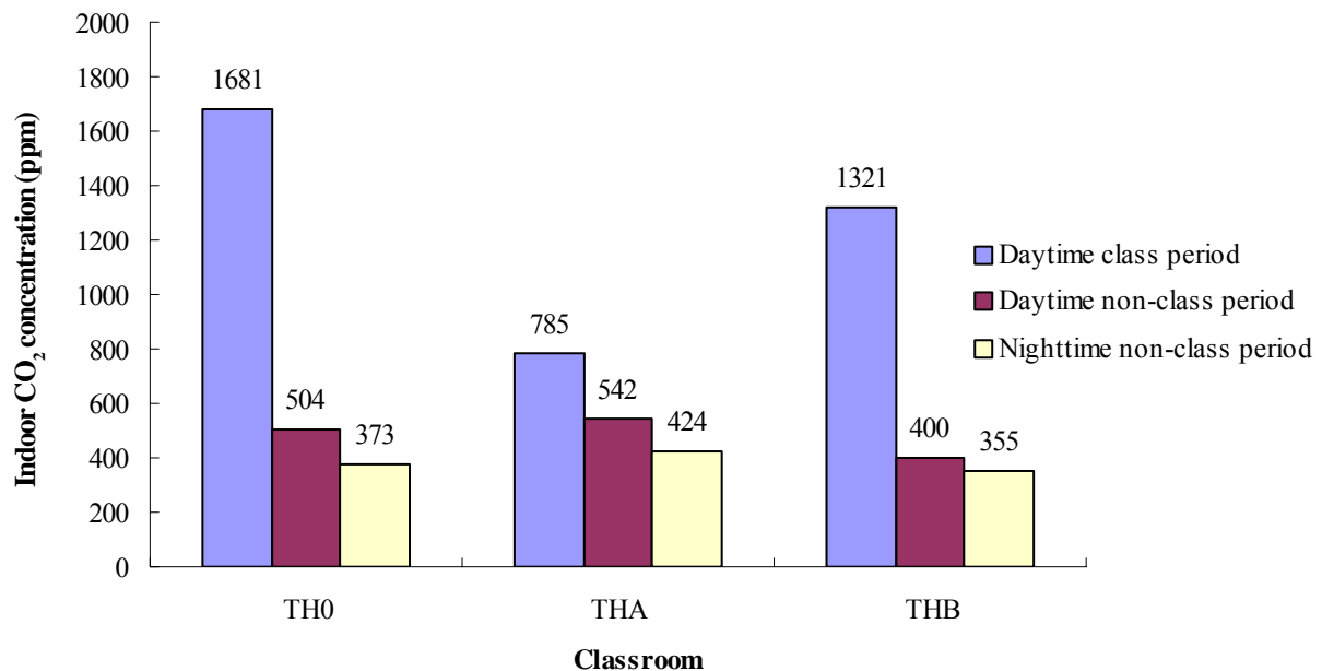
Fig. 1. Arithmetic means of indoor CO 2 concentrations according to classroom category and classes. For each classroom, the difference in indoor CO 2 concentrations according to classes was statistically significant (one-way ANOVA) ( p < 0.001 )
