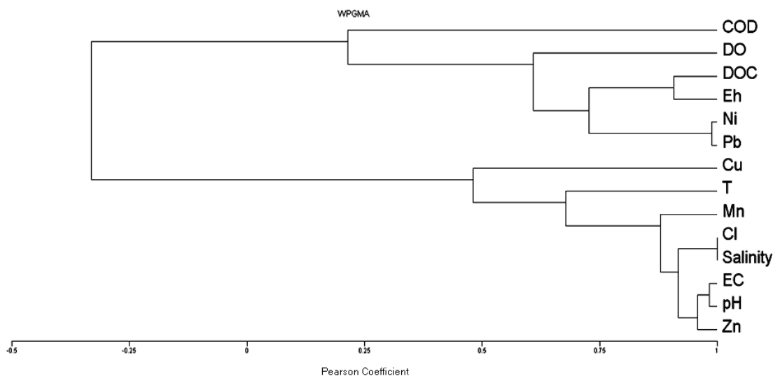
Fig. 1. Dendrogram of cluster analysis showing flocculation of metals and their governing factors
