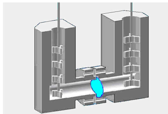
Fig. 2. Experiment Apparatus
