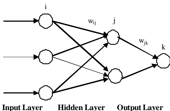
Fig. 1. A typical three-layer feed forward ANN
