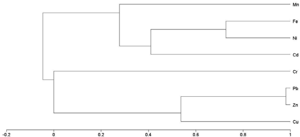
Fig. 3. Hierarchical cluster results or dendrogram obtained by CA of the sediment samples
