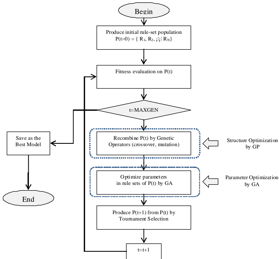
Fig. 2. Flowchart depicting the HEA application process.
