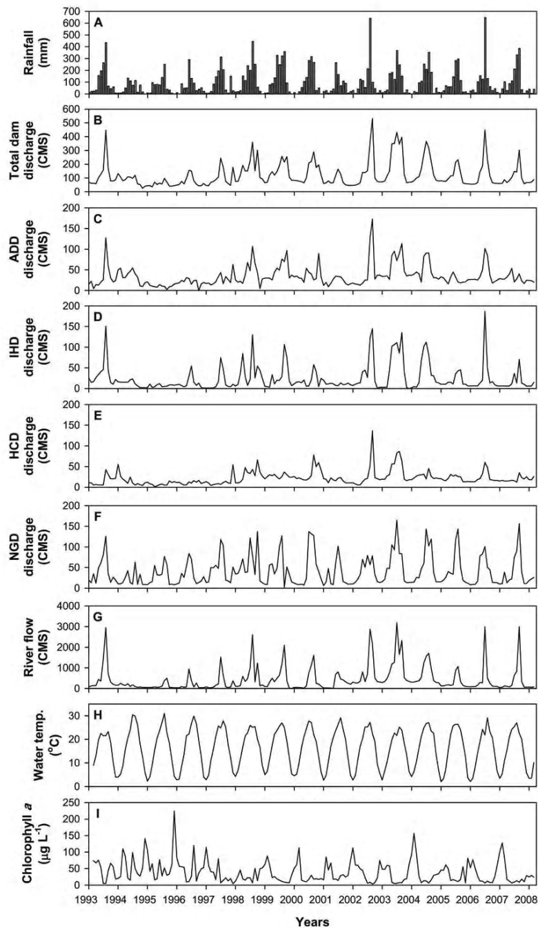
Fig. 3. Annual changes of meteorological, hydrological and water quality parameters. A, rainfall; B, total dam discharge; C, ADD discharge; D, IHD discharge; E, HCD discharge; F, NGD discharge; G, river flow; H, water temperature; I, chlorophyll a concentration.
