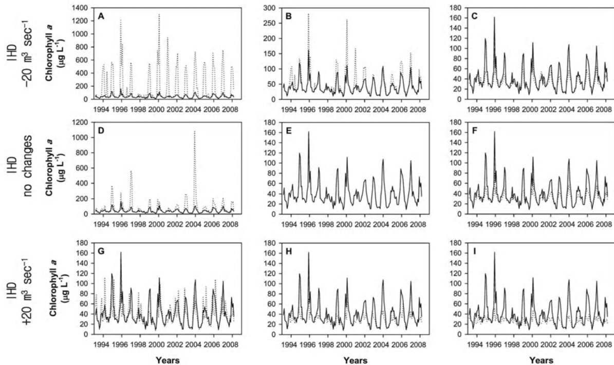
Fig. 7. Results of the brief scenario analysis changing the input of dam discharge by \pm 20 \text{ m}^3 \text{ sec}^{-1} in order to detect the response of chlorophyll a .
